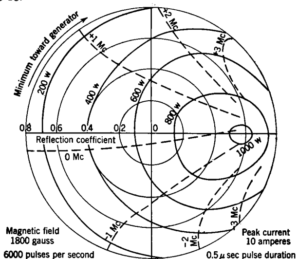
FIG. 19-34.—Rieke diagram for 2J41 magnetron.
